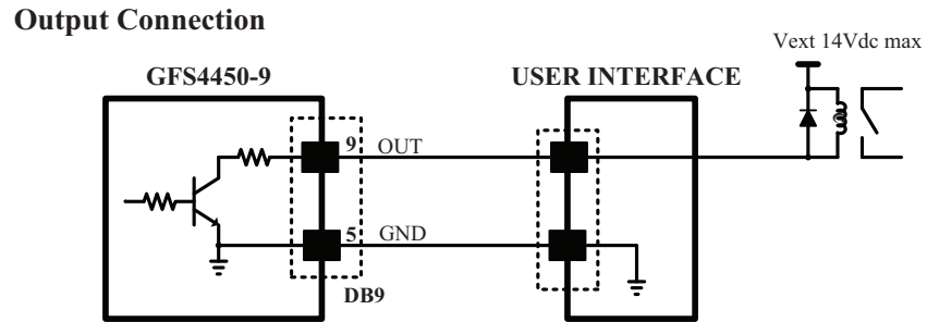
Figure 7. Output Connection
