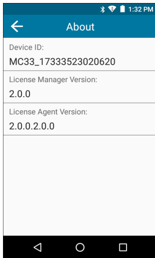
Figure 135 About Screen
