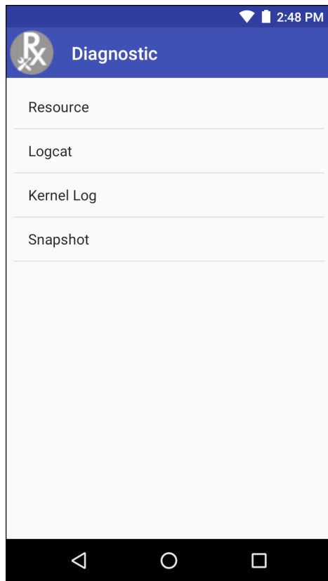
Figure 118 Diagnostic Window
