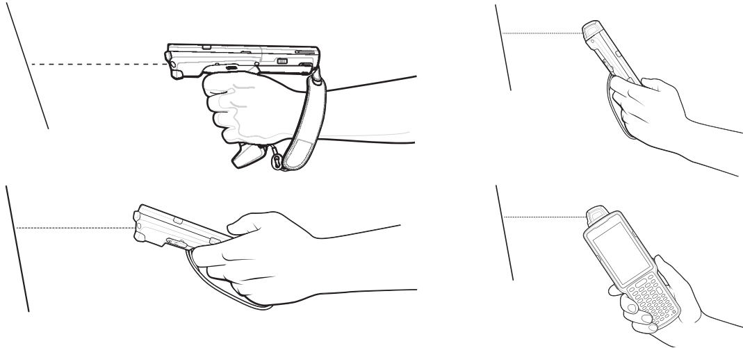
Figure 76 Data Capture
