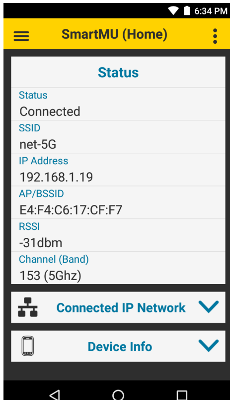
Figure 151 Home Screen
