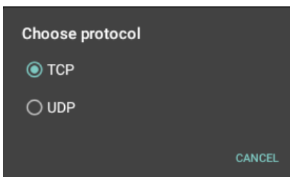
Figure 90 Protocol Selection
