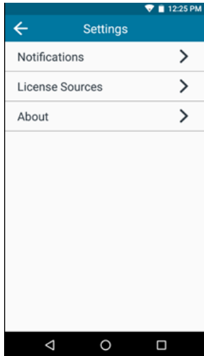
Figure 131 Settings Screen
