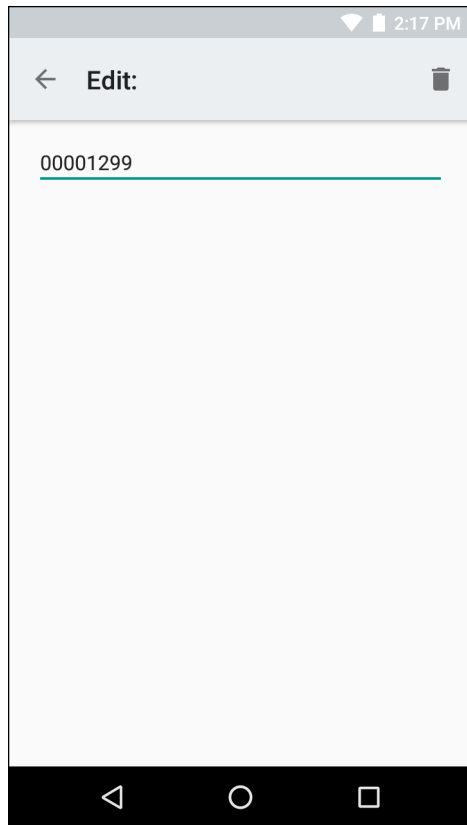
Figure 102 Formatted Data
