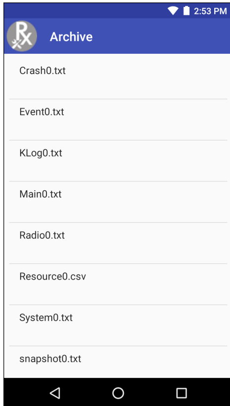
Figure 120 Archive
