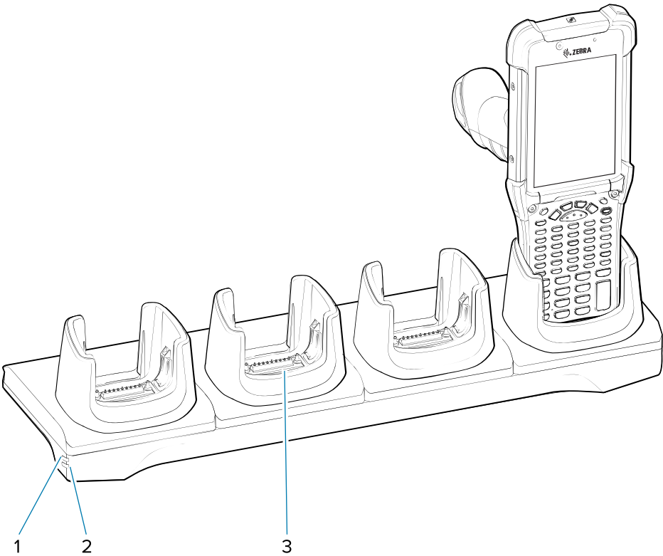
Figure 6 4-Slot Ethernet ShareCradle
